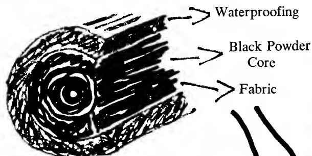
Figure 73. Safety fuse.
