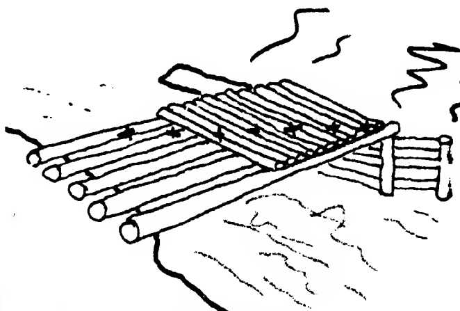
Figure 84. Slab bridge.
