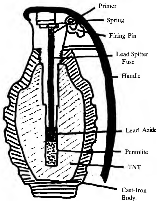
Figure 90. Military grenade.
