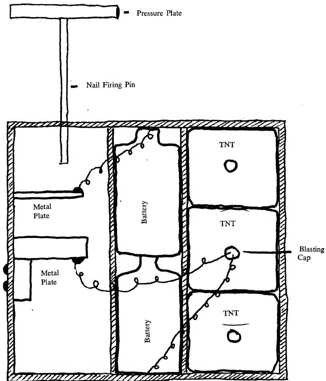
Figure 93. Pressure-plate detonator.
